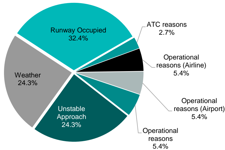
Figure 13: Reasons for go-arounds in 2021
